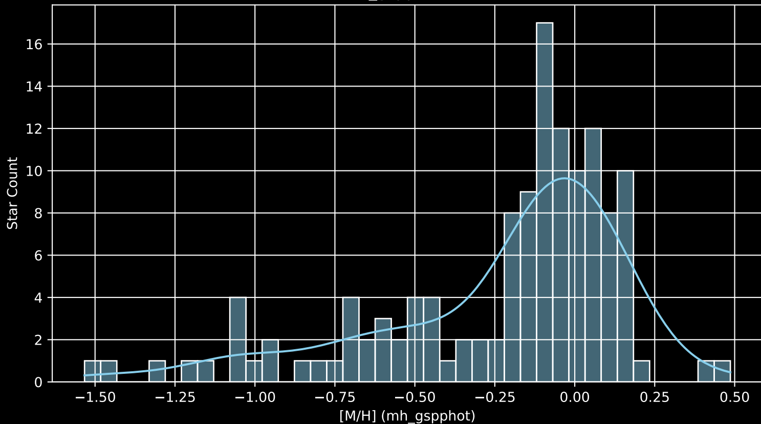
APOGEE DR17 Field: [000+14 [M/H] (mh_gspphot) (n= 130)
