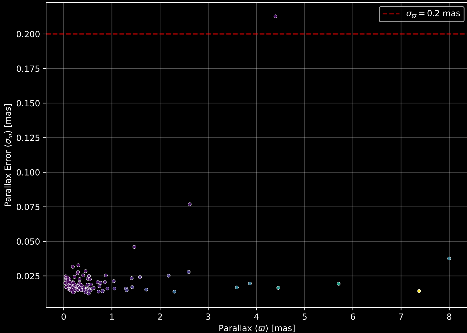
APOGEE DR17 Field: [000+14] Parallax Quality (n= 131)
