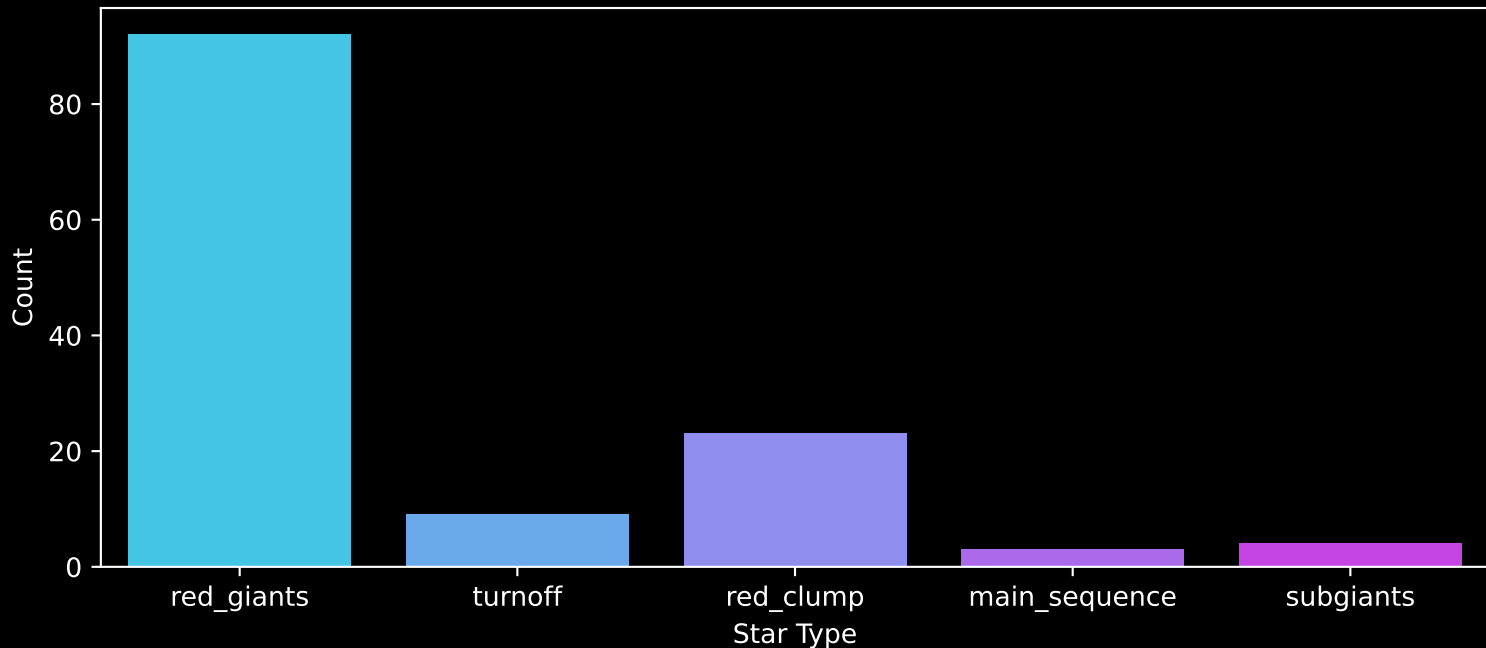
APOGEE DR17 Field: [000+14] Count plot of Star Type
