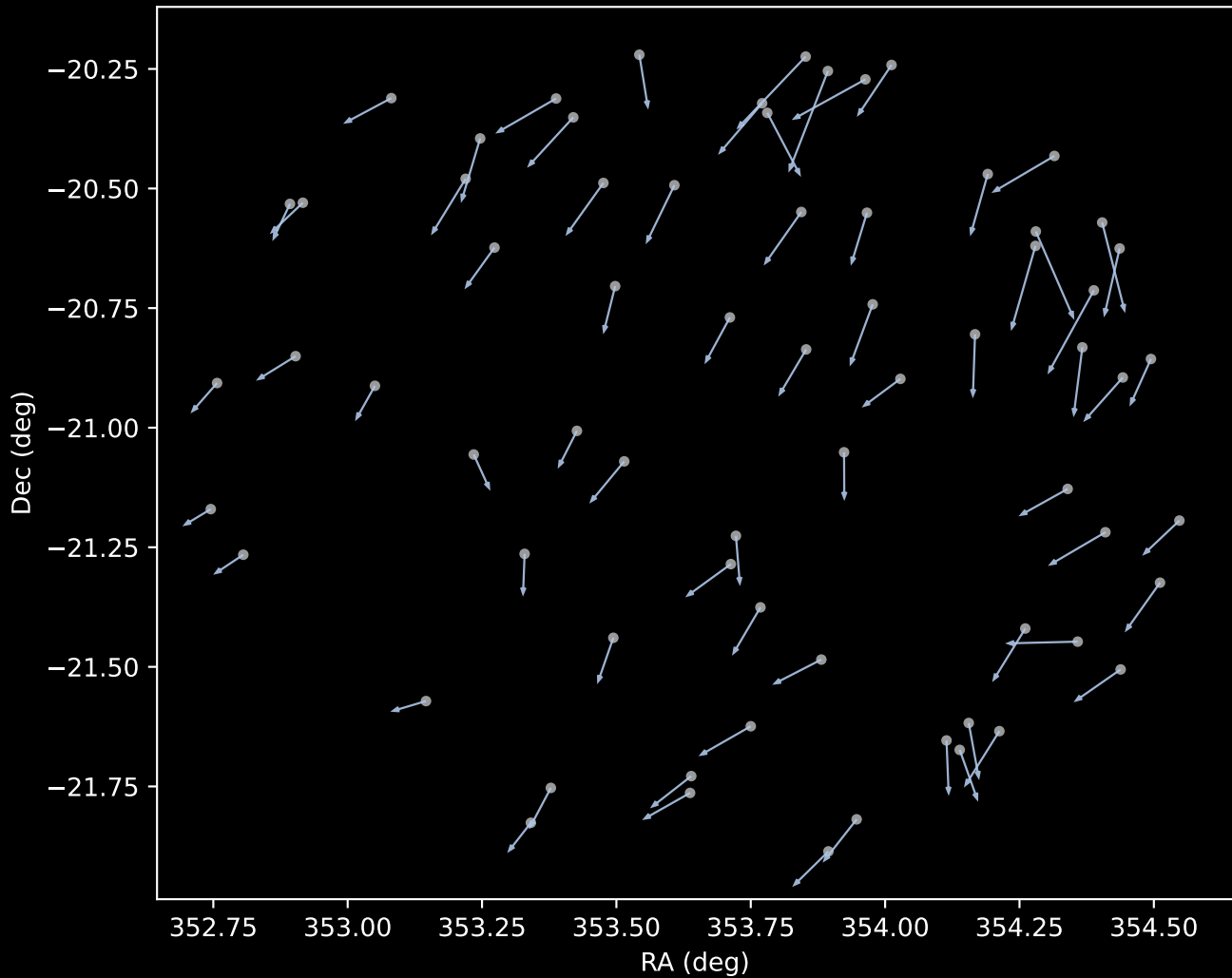
APOGEE DR17 Cluster 1 Proper Motion Vectors (n=69)
