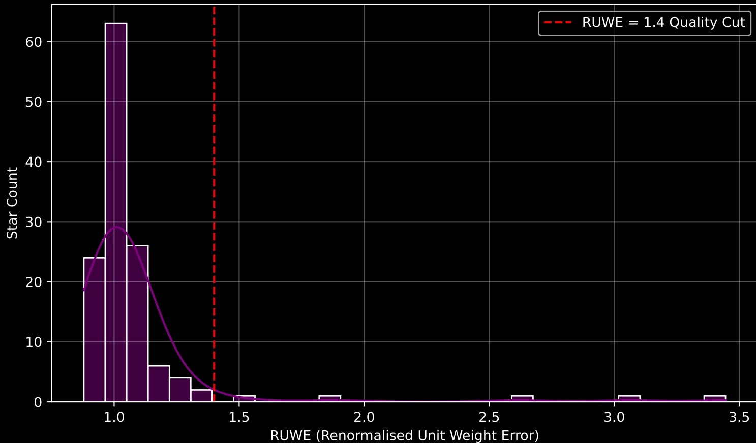
GAPOGEE DR17 Field [000+14] RUWE Distribution (n= 130)
