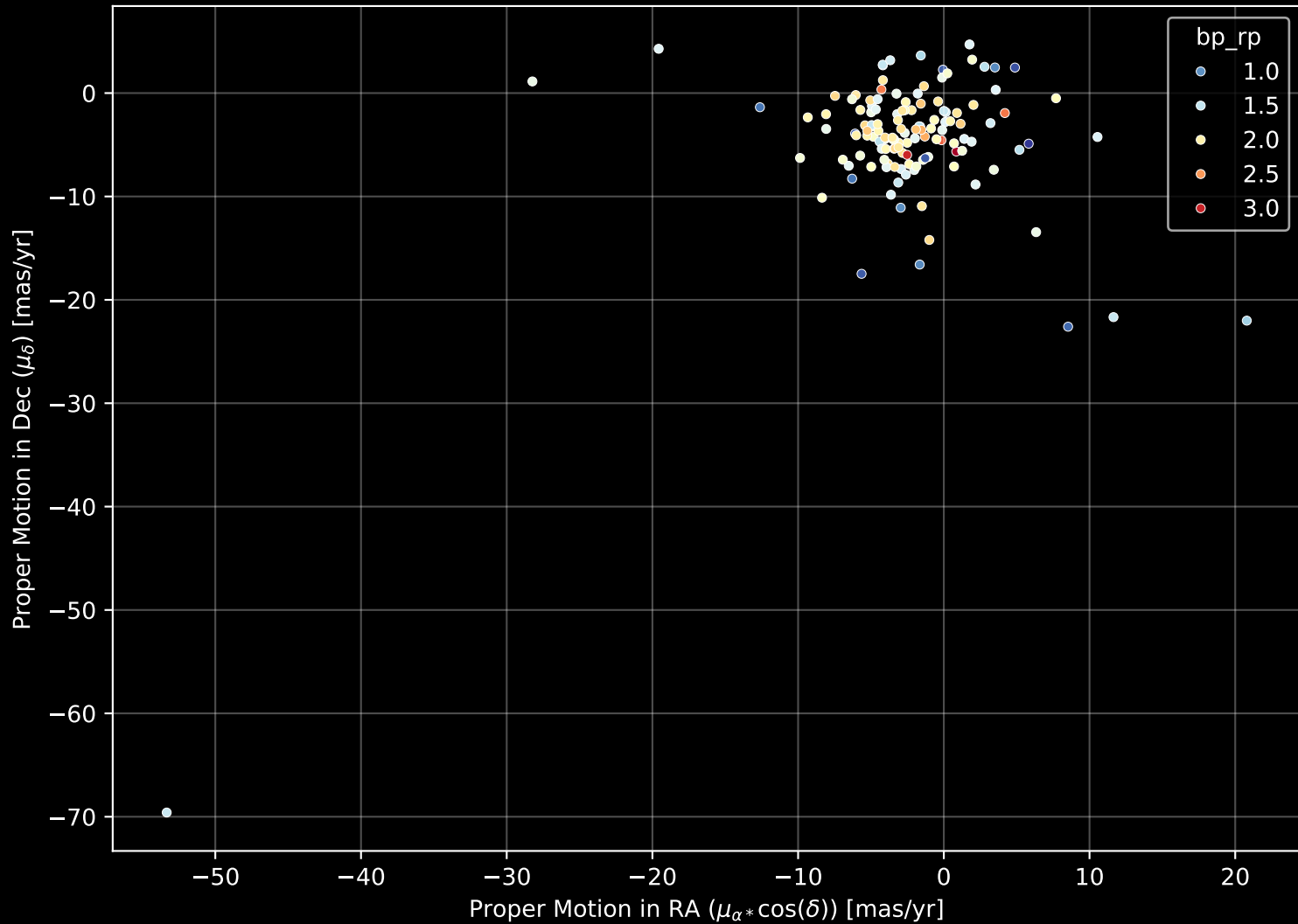
APOGEE DR17 Field: [000+14] Proper Motion Diagram (n= 131)
