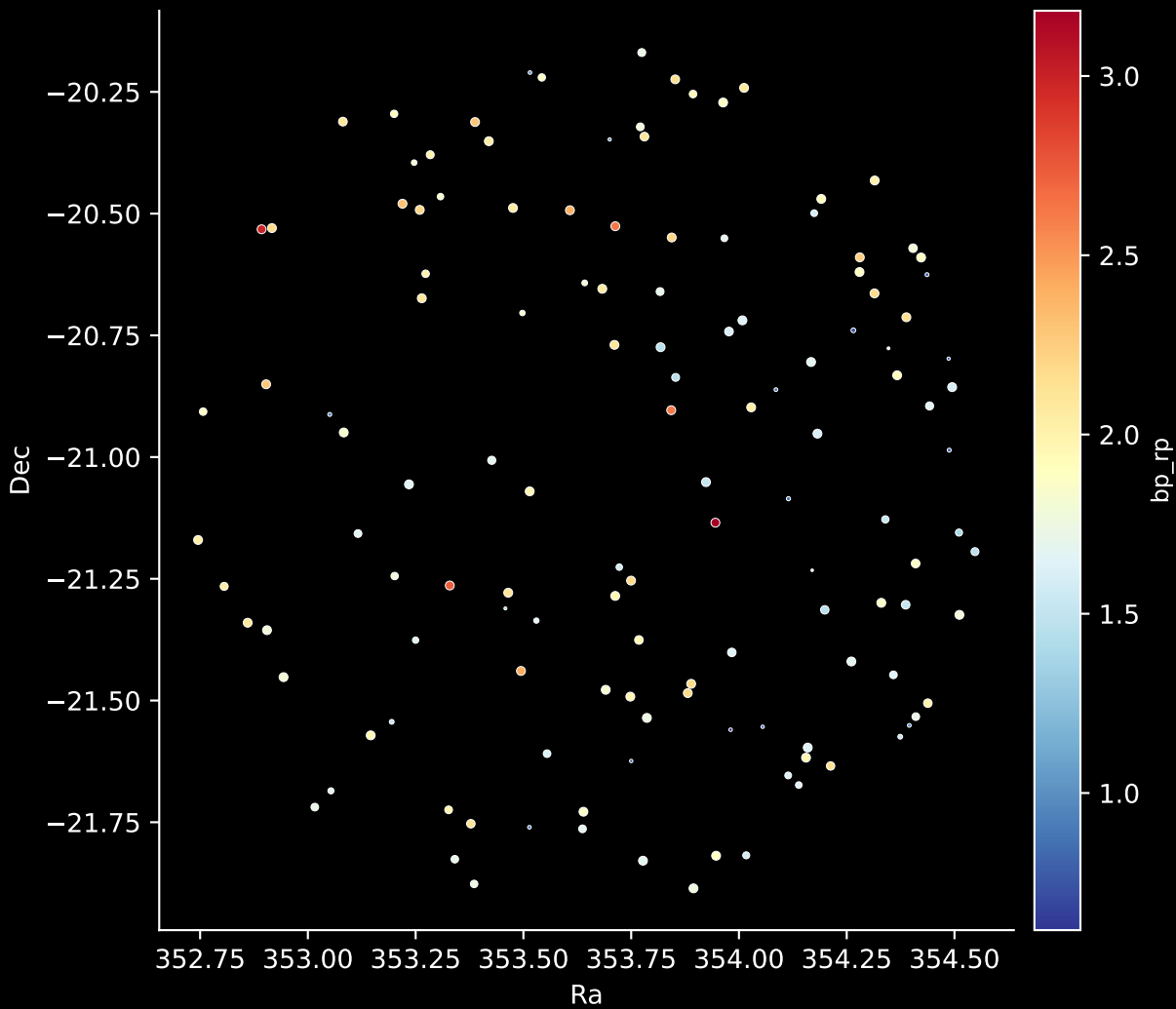
APOGEE DR17 Field: [000+14] Stars: 131
